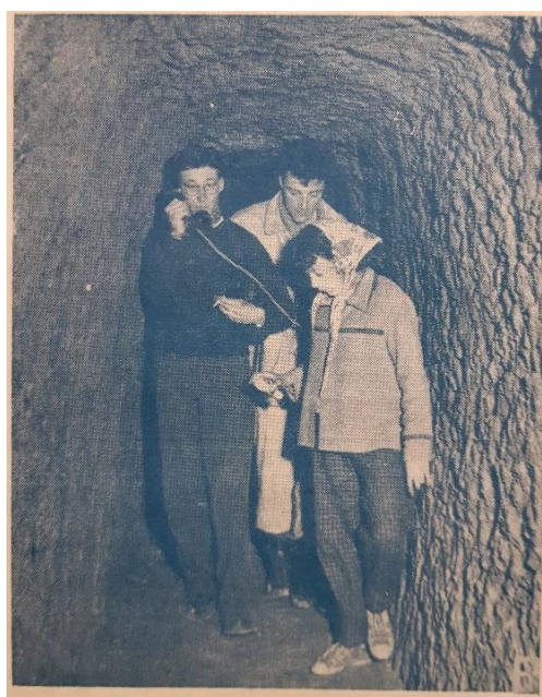
Figure 13: Left: Jean Evenou preparing a recording at the entrance of an abandoned gold mine in Brittany. His tape recorder is a Philips EL 3540. Note the truck battery in the forefront on the right, with the crocodile clips to link the battery to the recorder. Right: Christian Bodin, Georges Lequelllec and Yanette Evenou in the gold mine recording and commenting their expedition. Because the recorder was static at the entrance of the mine, and because the mine was huge, they relied on a telephone line to record their exploration. The telephone is clearly visible, held by Bodin.
