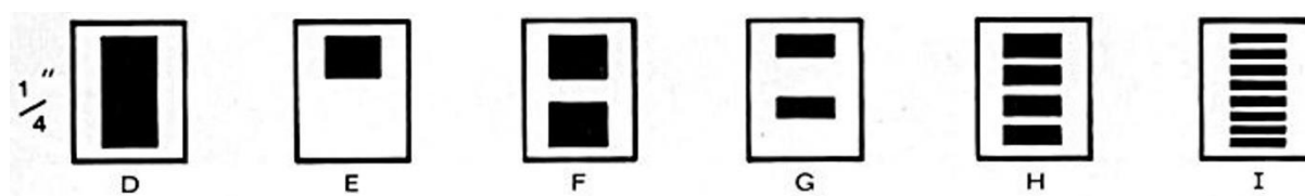
Figure 14: The different types of quarter inch tape heads, for recording and playback. The black squares are the surfaces of the electromagnets, that is to say, the surface on which the recording (or playback) will occur.
